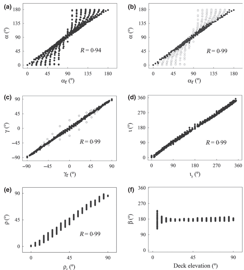
Figure 6. Calibration of the sensors. Correlation coefficients for the accelerometer [pitch angle ( \alpha , a–b) and roll angle ( \gamma , c)], magnetometer [midrib azimuth-angle ( \iota , d)], lamina inclination angle ( \rho ; e), and lamina course-angle ( \beta ; f). Unbiased (black) and biased (deviation from ideal correlation; white) values are shown for the pitch (a and b, respectively) and roll angle (c). Deviations from ideal correlation in 'a' and 'c' are minimized when accounting for the maximum slope angle (e). Lamina course-angle (f) was measured every 5^\circ from 5^\circ to vertical ( 90^\circ ). In Fig. 6a–e, n = 684 ; in Fig. 6f, n = 648 .
